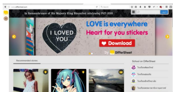
Fig. 2. DifferSheet.
